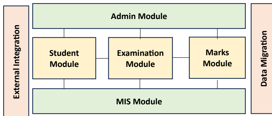
Figure-2: Proposed Modular Architecture
